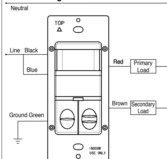
Single Power Source
