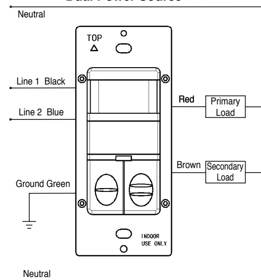
Dual Power Source
